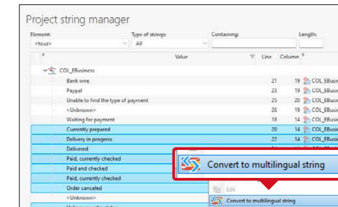
New multilingual string management window
