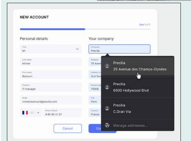
Result in the Browser
