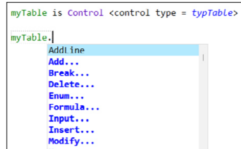
Code completion only shows functions for the Table control
