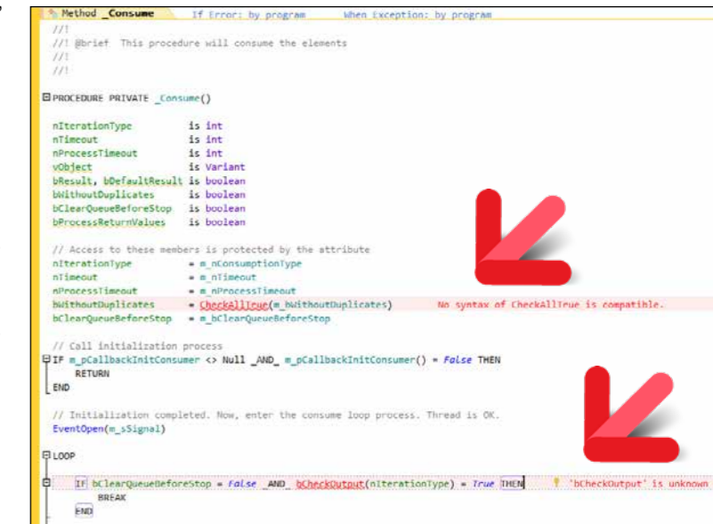
Programming errors and warnings are detailed directly in the code.
